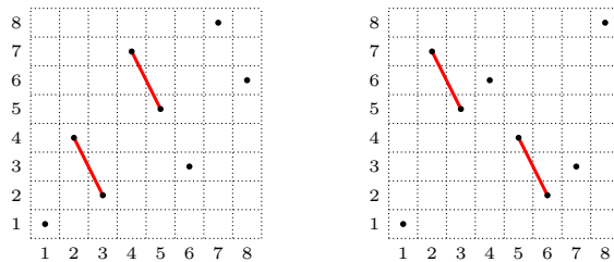
Figure 1: Two permutations \pi = 1\ 4\ 2\ 7\ 5\ 3\ 8\ 6 and \sigma = 1\ 7\ 5\ 6\ 4\ 2\ 3\ 8 in the same class with DD(\pi) = DD(\sigma) = \{(4, 2), (7, 5)\} .
